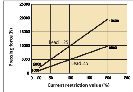
Correlation diagram of pressing force and current restriction value
