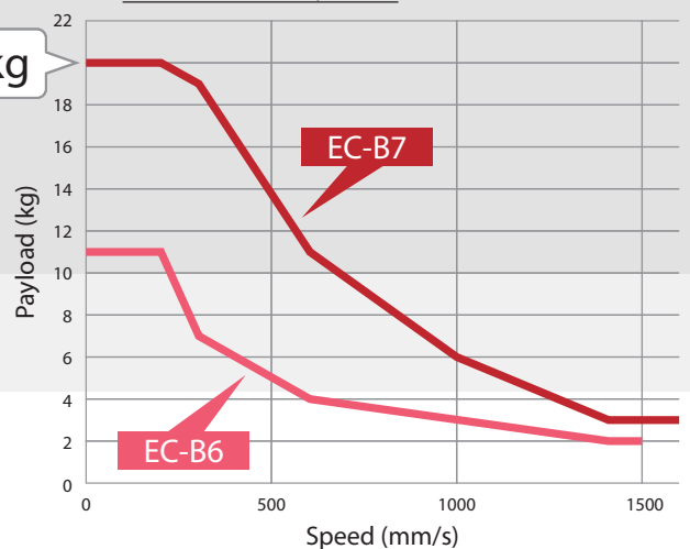
Correlation Diagram of Speed and Payload (Acceleration/deceleration: 0.3G)
